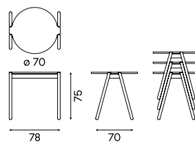
Stackable table
