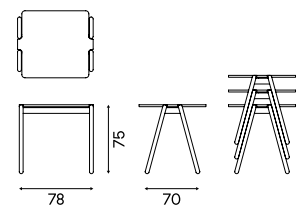
Stackable table
